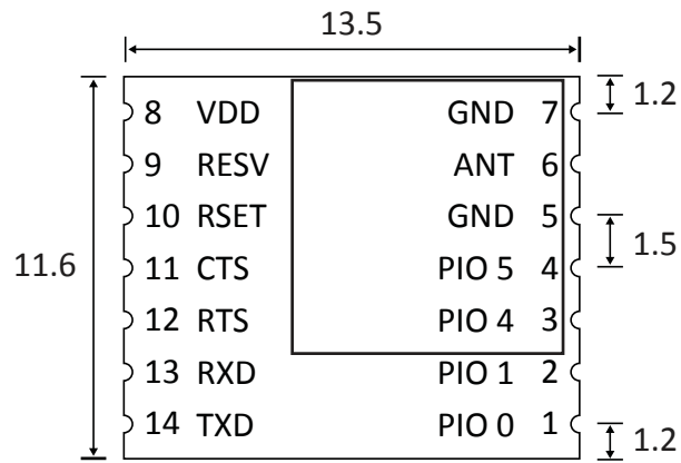
KC-22.5 Top View (dimensions in mm)
