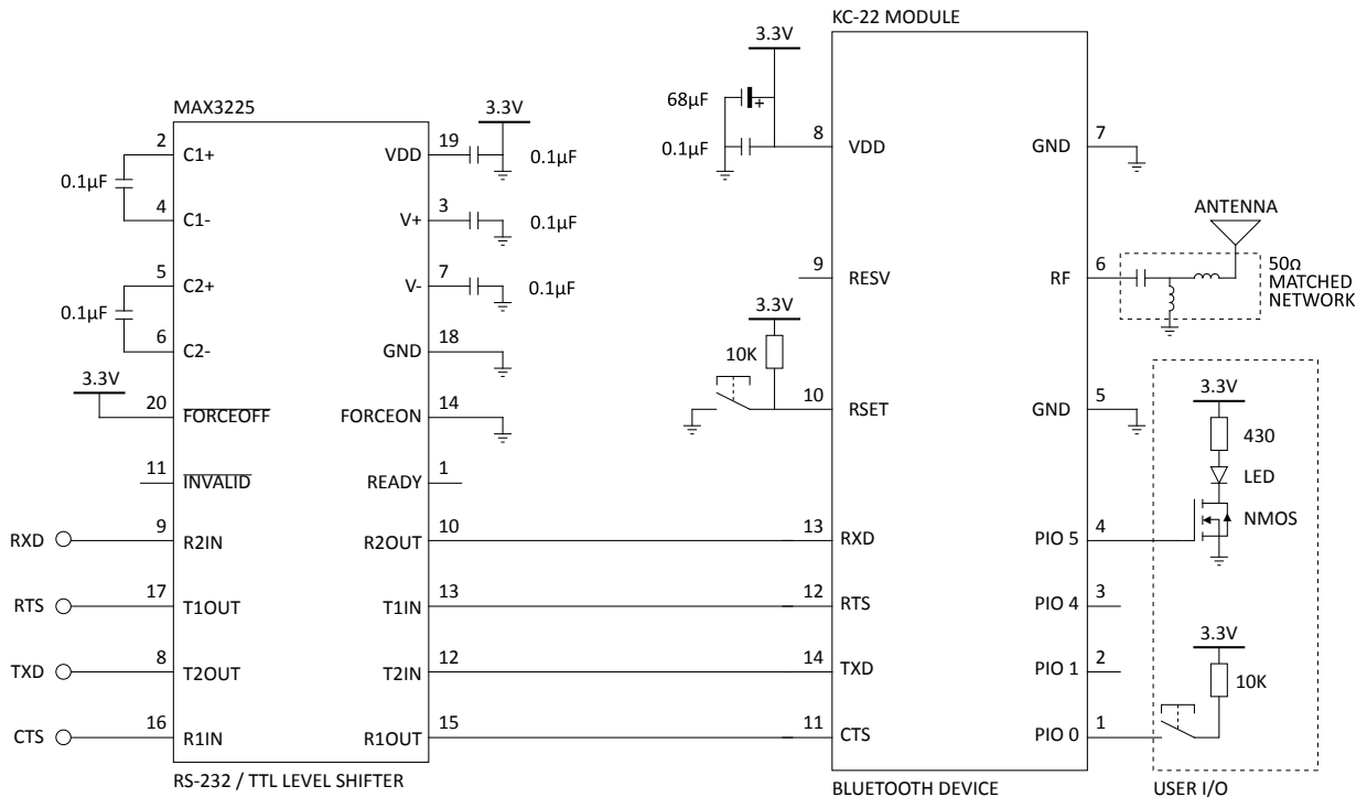
KC-22 sample circuit with TTL voltage level shifter ready to connect to a PC RS-232.
