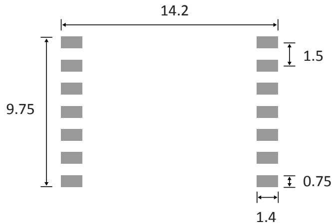
KC-22.5 Landing Pattern (dimensions in mm)
